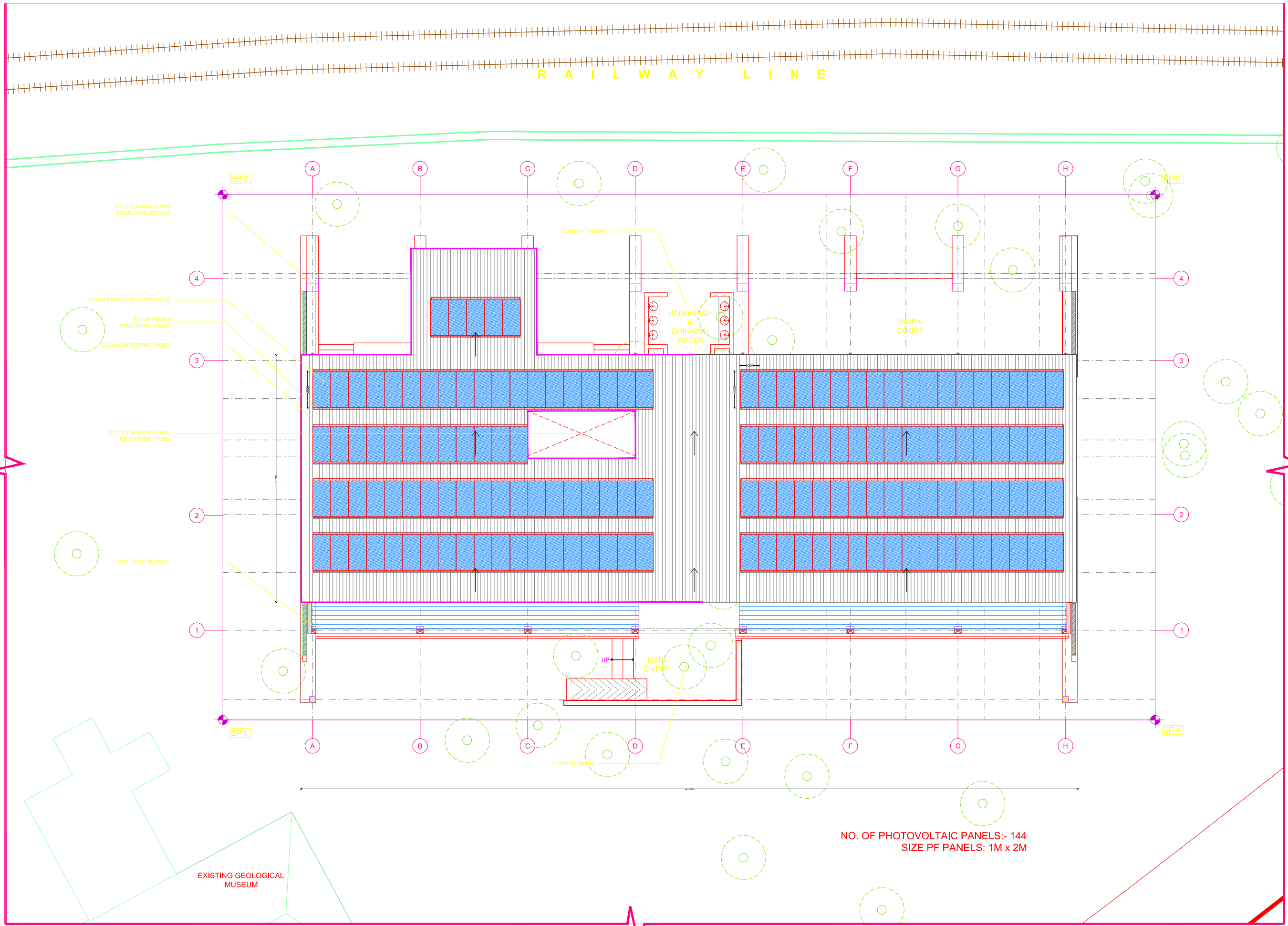
ROOF PLAN 1 1:100 204
