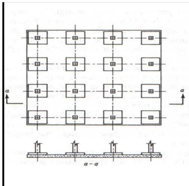
Raft Foundation
